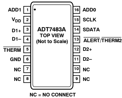
Figure 3.16-Lead QFN Pin Configuration
