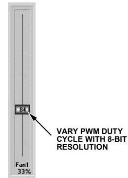
Figure 49. Control PWM Duty Cycle Manually with a Resolution of 0.39%
