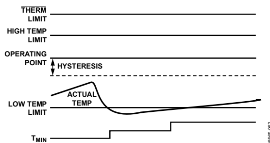
Figure 71. Increasing T_{\text{MIN}} for Quieter Operation
