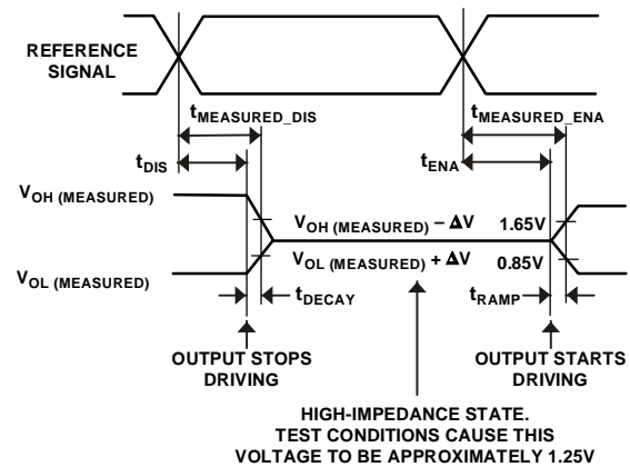
Figure 32. Output Enable/Disable
