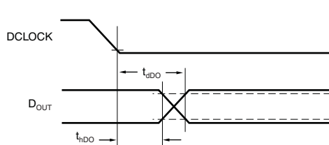
Voltage Waveforms for D_{OUT} Delay Times, t_{dDO}
