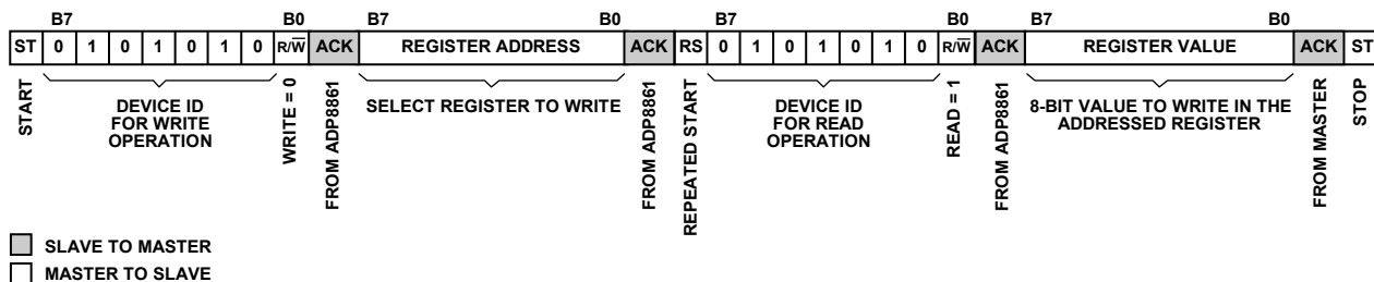
Figure 41. I 2 C Read Command Sequence
