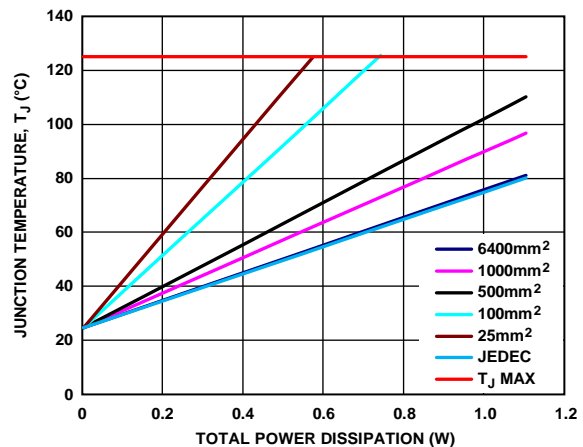
Figure 89. Junction Temperature vs. Total Power Dissipation for the 8-Lead LFCSP, T_A = 25^\circ\text{C}
