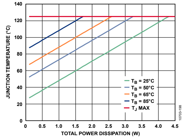
Figure 99. Junction Temperature vs. Total Power Dissipation for the 6-Lead LFCSP, T_A = 85^\circ\text{C}
