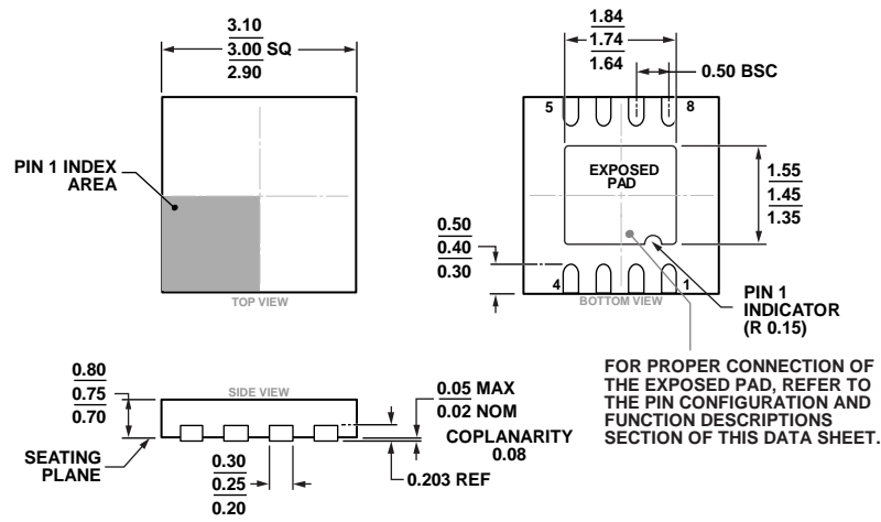
COMPLIANT TO JEDEC STANDARDS MO-229-WEED-4 Figure 105. 8-Lead Lead Frame Chip Scale Package [LFCSP] 3 mm x 3 mm Body and 0.75 Package Height (CP-8-13) Dimensions shown in millimeters
