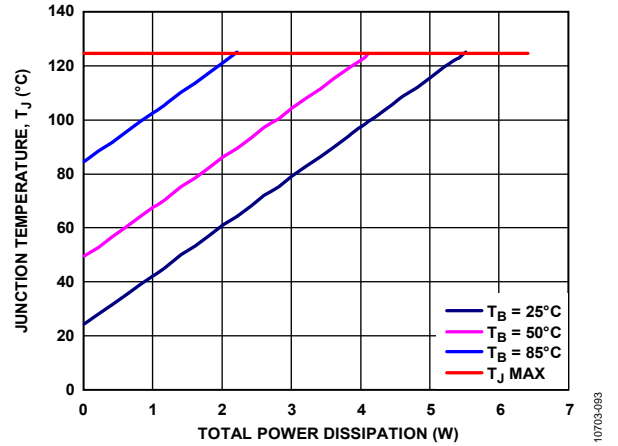
Figure 98. Junction Temperature vs. Total Power Dissipation for the 8-Lead LFCSP, T_A = 85^\circ\text{C}
