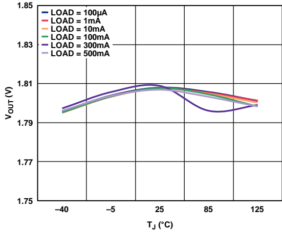
Figure 23. Output Voltage vs. Junction Temperature, V_{OUT} = 1.8\text{ V}
