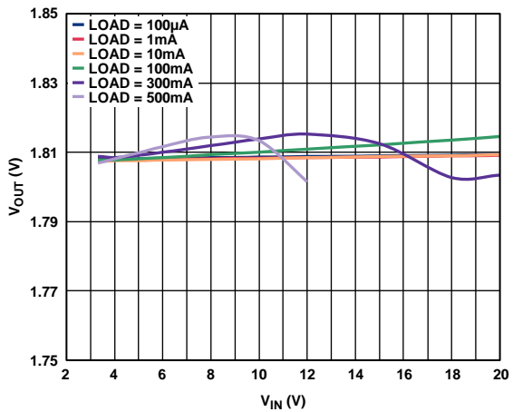
Figure 25. Output Voltage vs. Input Voltage, V_{OUT} = 1.8\text{ V}
