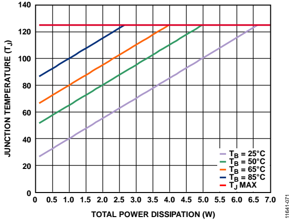
Figure 77. LFCSP
