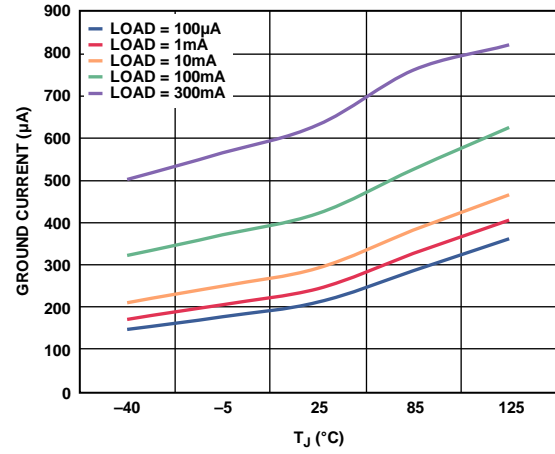
Figure 26. Ground Current vs. Junction Temperature, V_{OUT} = 1.8\text{ V}
