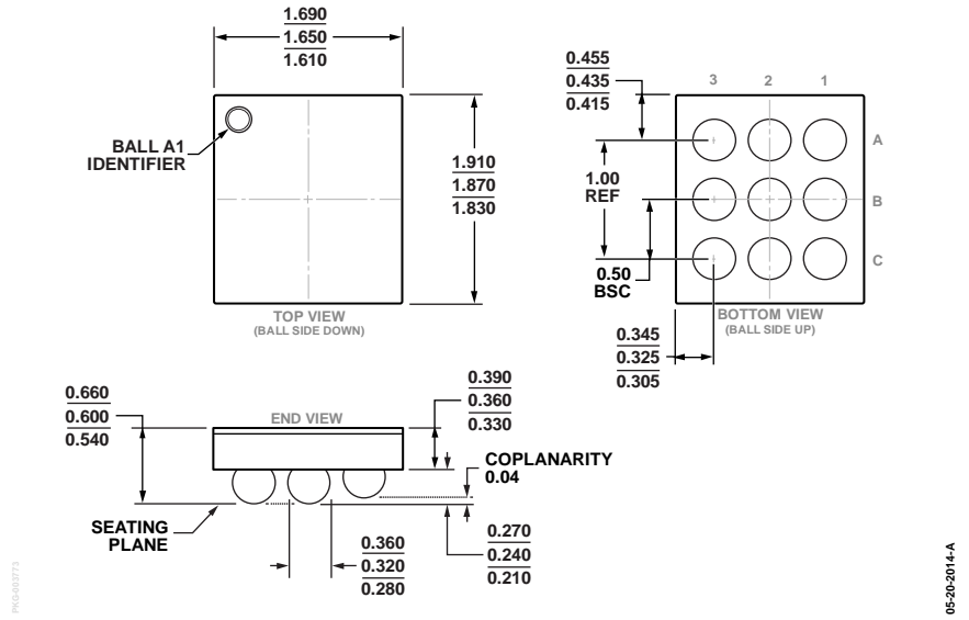
Figure 42. 9-Ball Wafer Level Chip Scale Package [WLCSP] (CB-9-6) Dimensions shown in millimeters
