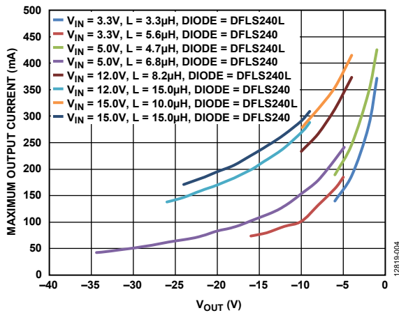
Figure 4. Maximum Output Current, f_{SW} = 2.4 MHz, T_A = 25^\circ\text{C} , Based on Target of 70% I_{LIM}
