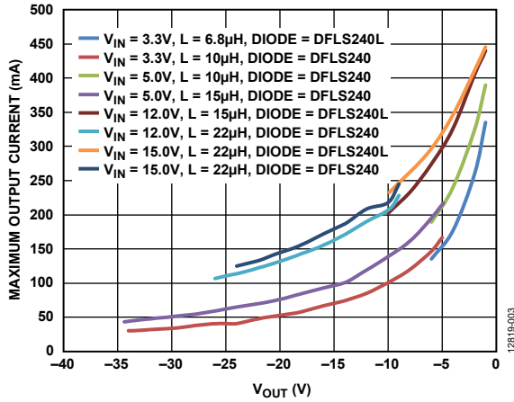
Figure 3. Maximum Output Current, f_{SW} = 1.2 MHz, T_A = 25^\circ\text{C} , Based on Target of 70% I_{LIM}
