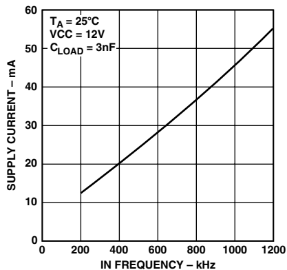
TPC 7. Supply Current vs. Frequency
