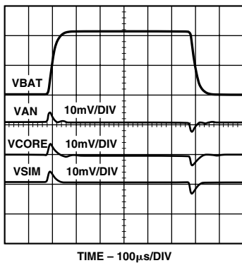
TPC 7. Line Transient Response, Minimum Loads
