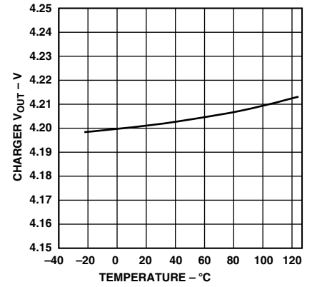
TPC 21. Charger V_{OUT} vs. Temperature, V_{IN} = 5.0\text{ V} , I_{LOAD} = 10\text{ mA}
