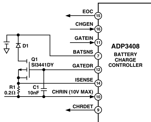
Figure 2. Battery Charger Typical Application
