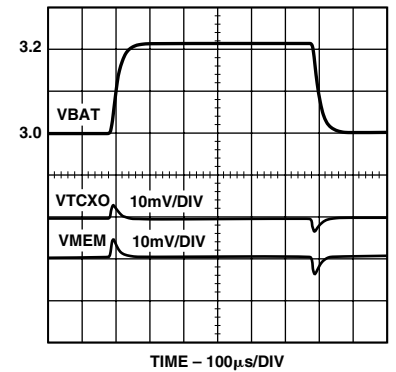
TPC 6. Line Transient Response, Maximum Loads
