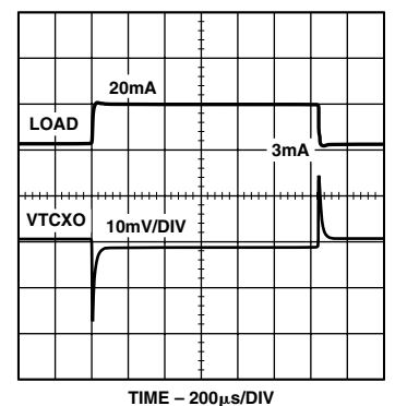
TPC 9. VTCXO Load Step
