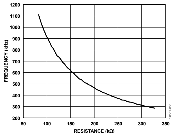
Figure 56. Frequency vs. Resistance
