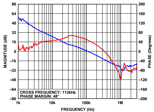
Figure 39. ADP2119 Bode Plot at V_{IN} = 5\text{V} , V_{OUT} = 1.5\text{V} , I_o = 2\text{A} , L = 1.5\mu\text{H} , C_{OUT} = 22\mu\text{F} + 10\mu\text{F}
