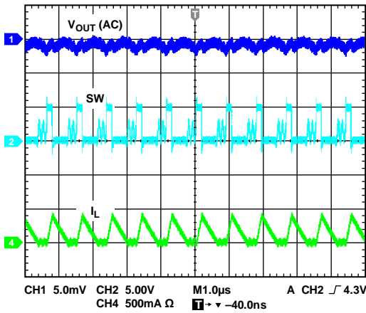
Figure 35. Discontinuous Conduction Mode (DCM)
