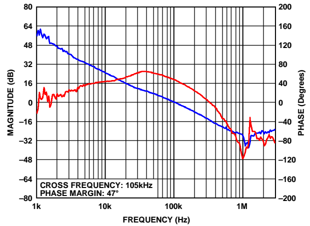
Figure 38. ADP2119 Bode Plot at V_{IN} = 5\text{V} , V_{OUT} = 1.2\text{V} , I_o = 2\text{A} , L = 1.5\mu\text{H} , C_{OUT} = 2 \times 22\mu\text{F}
