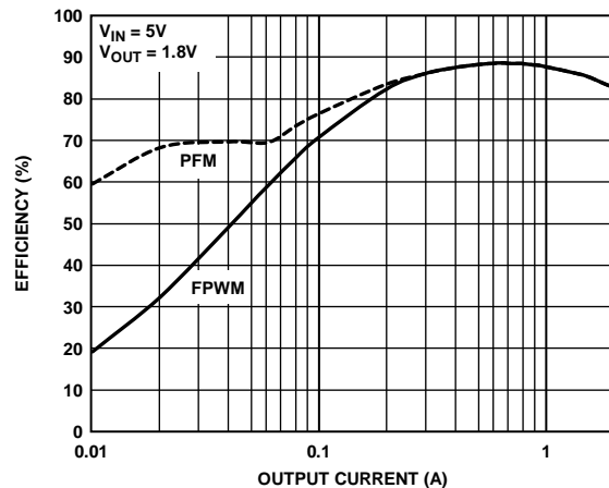
Figure 2. ADP2119 Efficiency vs. Output Current
