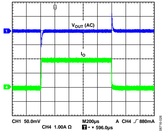
Figure 26. Load Transient (ADP2119, FPWM, V_{IN} = 5\text{ V} )
