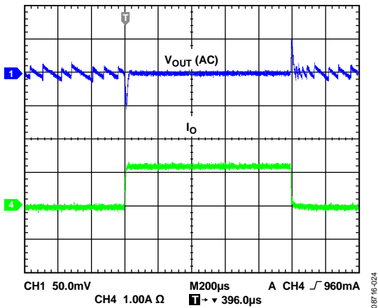
Figure 24. Load Transient (ADP2120, PFM, V_{IN} = 5\text{ V} )
