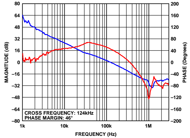
Figure 37. ADP2119 Bode Plot at V_{IN} = 5\text{V} , V_{OUT} = 1.0\text{V} , I_o = 2\text{A} , L = 1\mu\text{H} , C_{OUT} = 2 \times 22\mu\text{F}
