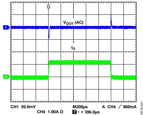
Figure 27. Load Transient (ADP2120, FPWM, V_{IN} = 5\text{ V} )
