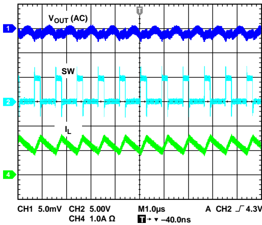
Figure 36. Continuous Conduction Mode (CCM)
