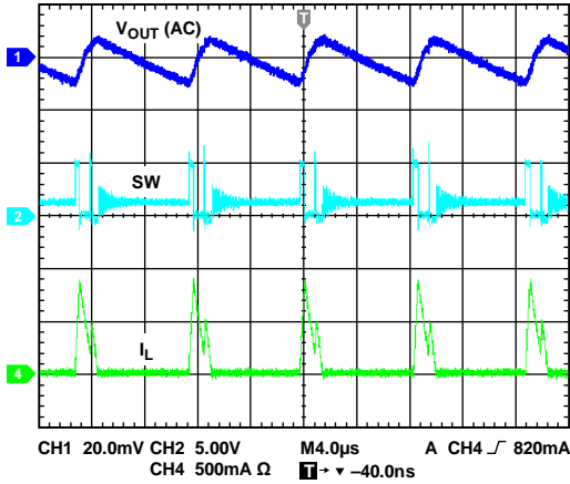
Figure 34. PFM Mode
