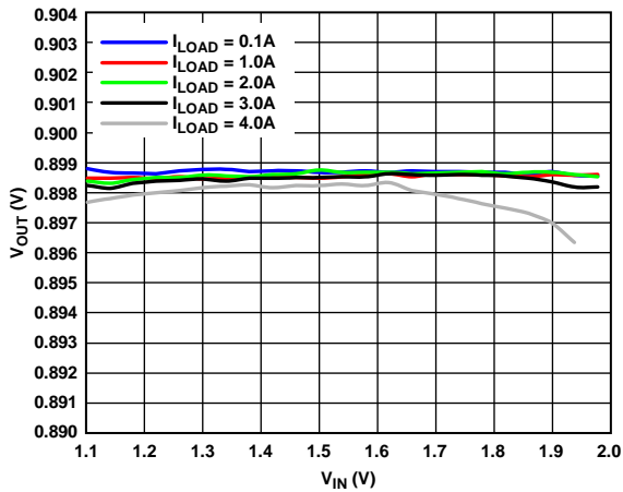
Figure 12. Output Voltage ( V_{OUT} ) vs. Input Voltage ( V_{IN} ), V_{OUT} = 0.9\text{ V}
