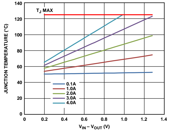
Figure 55. 100 mm 2 of PCB Copper, T_B = 50^\circ\text{C} , LFCSP
