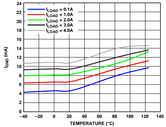
Figure 13. Ground Current ( I_{GND} ) vs. Temperature, V_{OUT} = 0.9\text{ V}
