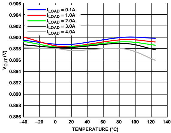
Figure 10. Output Voltage ( V_{OUT} ) vs. Temperature, V_{OUT} = 0.9\text{ V}
