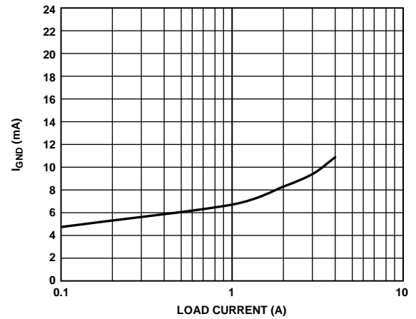
Figure 14. Ground Current ( I_{GND} ) vs. Load Current ( I_{LOAD} ), V_{OUT} = 0.9\text{ V}
