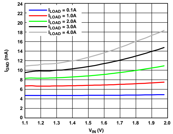
Figure 15. Ground Current ( I_{GND} ) vs. Input Voltage ( V_{IN} ), V_{OUT} = 0.9\text{ V}
