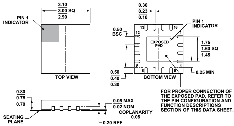
Figure 49. 16-Lead Lead Frame Chip Scale Package [LFCSP] 3 mm x 3 mm Body and 0.75 mm Package Height (CP-16-22)
