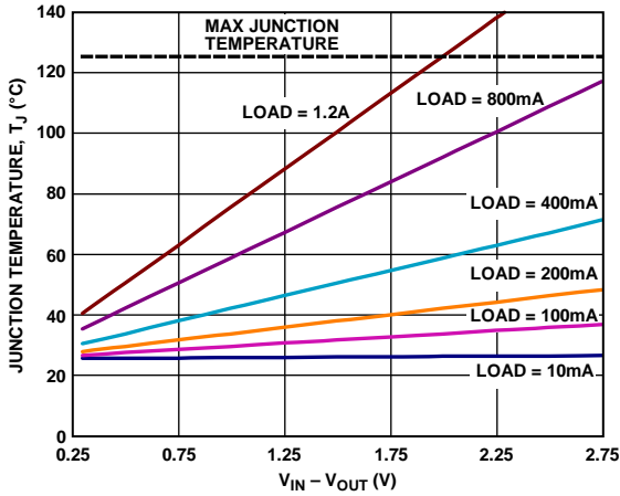
Figure 36. 6400 mm 2 of PCB Copper, T A = 25°C, LFCSP
