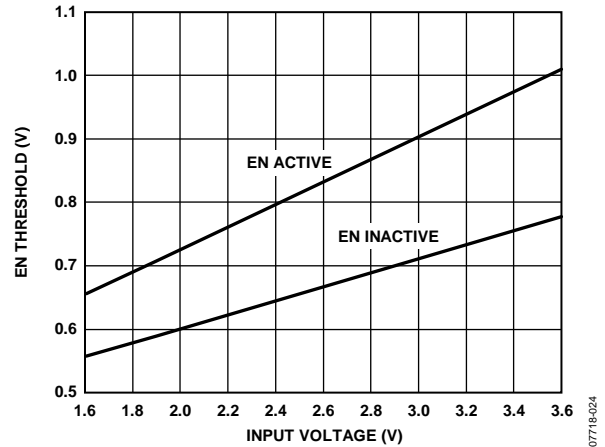
Figure 29. Typical EN Pin Thresholds vs. Input Voltage
