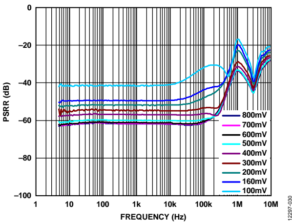
Figure 30. Power Supply Rejection Ratio (PSRR) vs. Frequency, V_{OUT} = 3 V , 500 mA Load Current, Various Headroom Voltages
