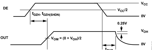
Figure 10. Driver Enable and Disable Times ( t_{DZH} , t_{DZH} , t_{DZH(SHDN)} )
