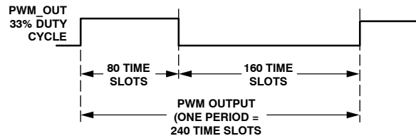
Figure 27. 33% PWM Duty Cycle Presented in Time Slots
