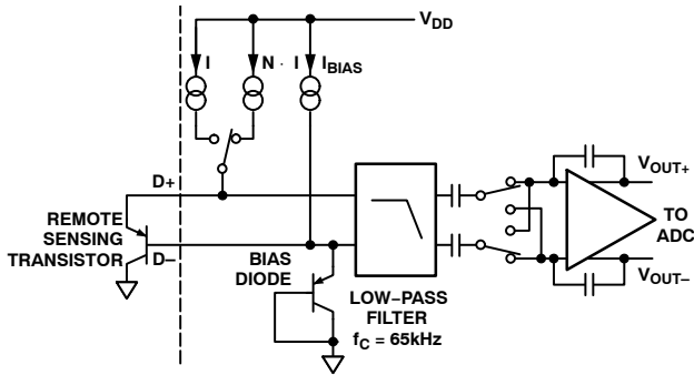
Figure 18. Signal Conditioning
