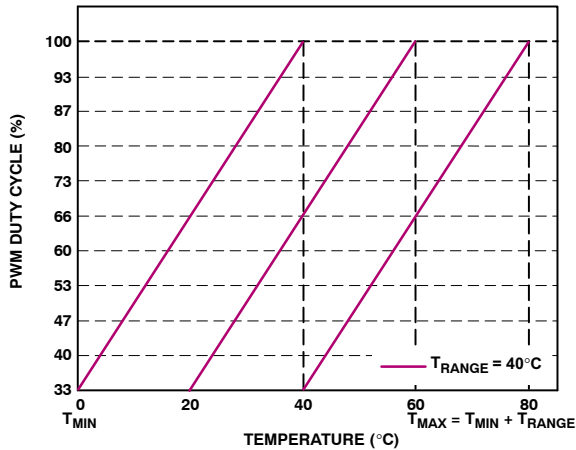
Figure 23. Effect of Increasing T_{MIN} Value on Control Loop
