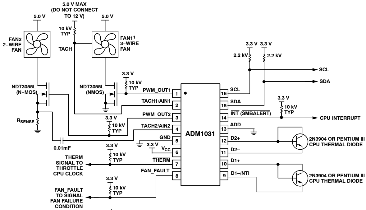
1 IN ACTUAL APPLICATION, BOTH FANS MUST BE 2-WIRE OR 3-WIRE TYPE. A SINGLE BIT CONTROLS WHETHER TACH1/AIN1 AND TACH2/AIN2 ARE ANALOG OR DIGITAL INPUTS.
