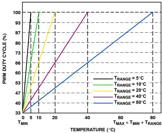
Figure 22. PWM Duty Cycle vs. Temperature Slope ( T_{RANGE} )
