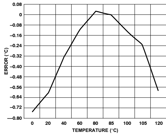
Figure 12. Remote Temperature Sensor Error
