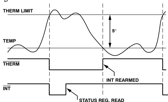
Figure 20. Operation of THERM and INT Signals
