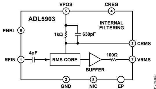
Figure 39. Simplified Architecture
