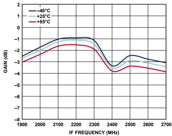
Figure 81. Power Conversion Gain vs. IF Frequency
