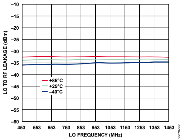
Figure 69. LO to RF Leakage vs. LO Frequency
