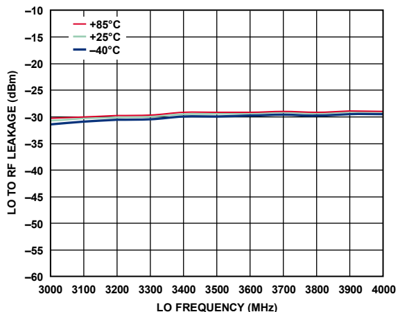
Figure 47. LO to RF Leakage vs. LO Frequency
