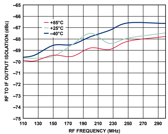
Figure 80. RF to IF Output Isolation vs. RF Frequency
