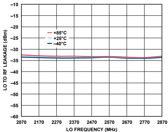
Figure 79. LO to RF Leakage vs. LO Frequency
