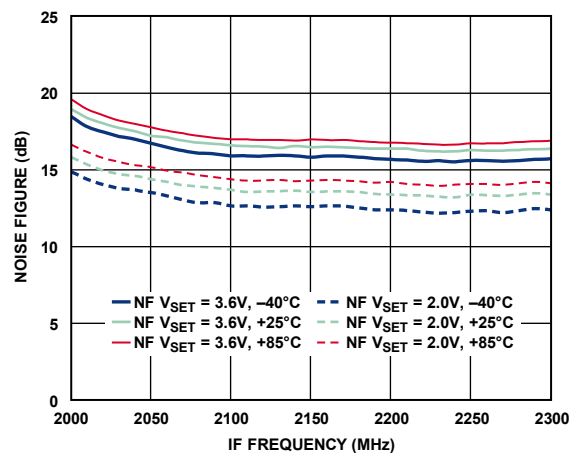
Figure 77. Noise Figure vs. IF Frequency, F_{LO} = 1950 MHz
