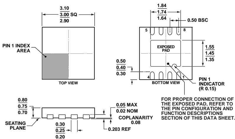
Figure 27. 8-Lead Lead Frame Chip Scale Package [LFCSP_WD] 3 mm × 3 mm Body, Very Very Thin, Dual Lead (CP-8-13)
