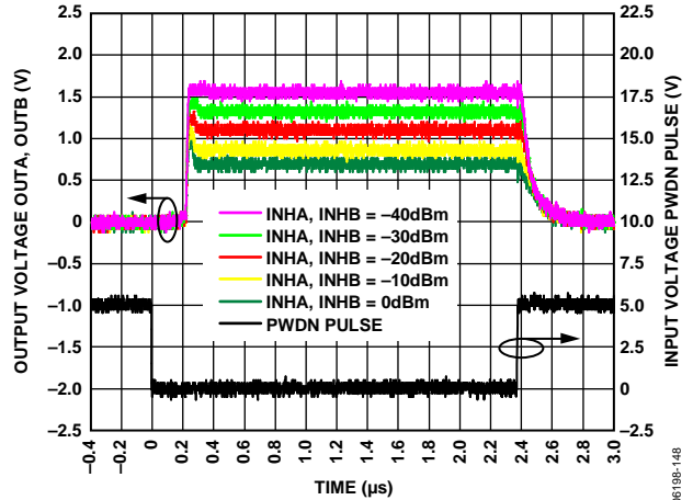
Figure 48. Output Response Using Power-Down Mode for Various RF Input Levels, Carrier Frequency = 900 MHz, CLPA = 0.1 µF
