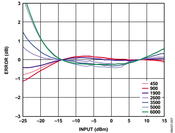
Figure 7. Linearity Error vs. Input Level, 450 MHz, 900 MHz, 1900 MHz, 2600 MHz, 3500 MHz, 5000 MHz, 6000 MHz Frequencies, 3.0 V Supply
