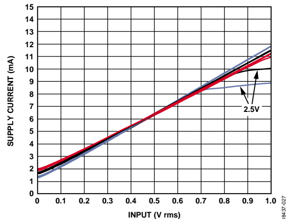
Figure 27. Supply Current vs. Input Level, 2.5 V, 3.0 V, and 3.3 V Supplies, 900 MHz Frequency, at -40^{\circ}C , +25^{\circ}C , and +85^{\circ}C
