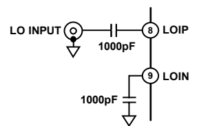
Figure 46. Single-Ended LO Drive
