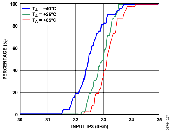
Figure 27. IIP3 Distributions
