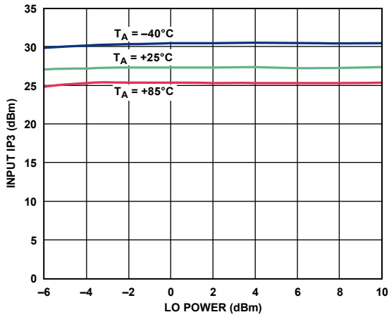
Figure 22. Input IP3 vs. LO Power
