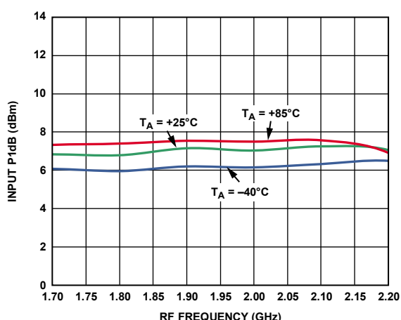
Figure 49. Input P1dB vs. RF Frequency at 3.3 V
