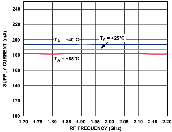
Figure 3. Supply Current vs. RF Frequency
