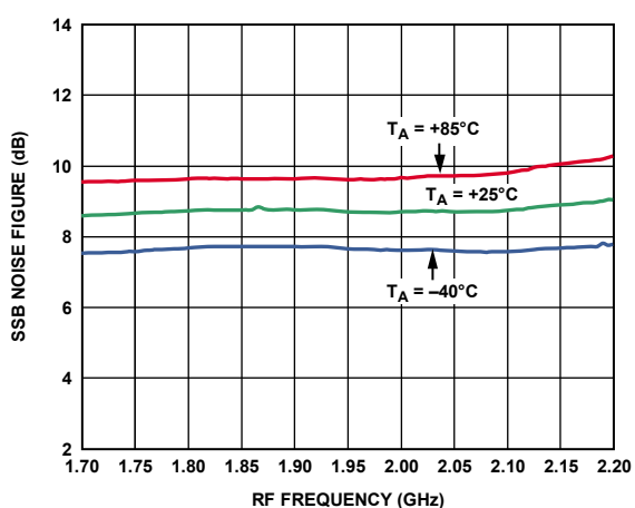
Figure 50. SSB Noise Figure vs. RF Frequency at 3.3 V
