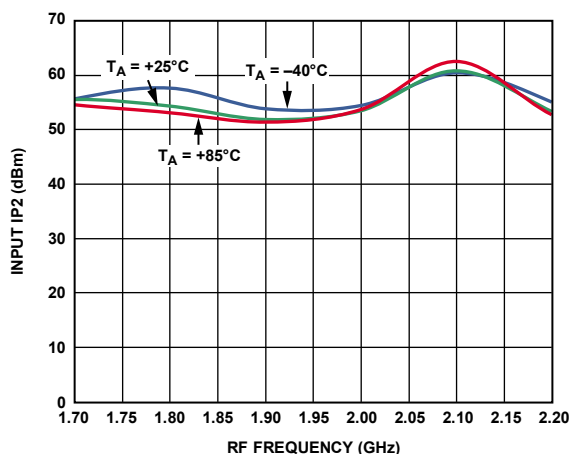
Figure 48. Input IP2 vs. RF Frequency at 3.3 V
