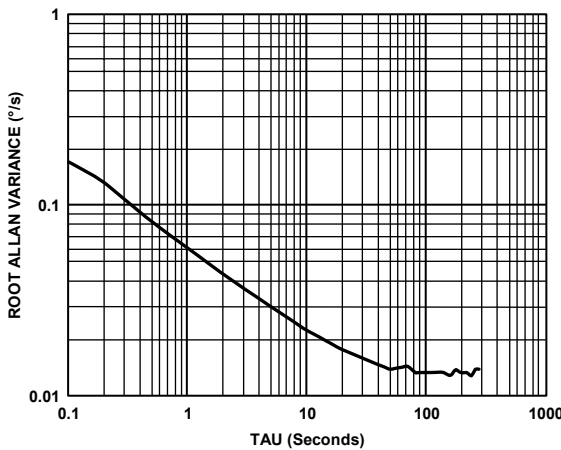
Figure 9. Root Allan Variance vs. TAU
