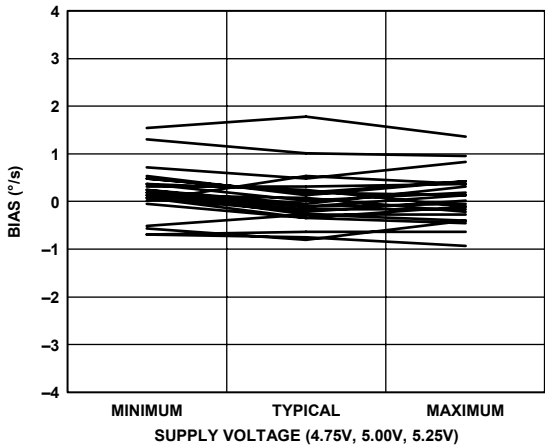
Figure 8. Bias vs. Supply Voltage
