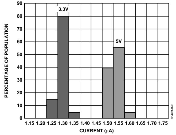
Figure 21. Supply Current at 25°C
