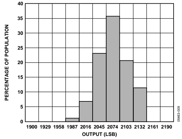
Figure 10. X-Axis Zero g Bias at 25°C
