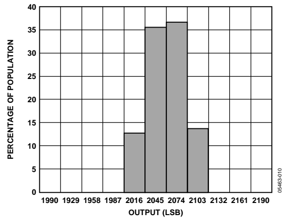
Figure 11. Y-Axis Zero g Bias at 25°C
