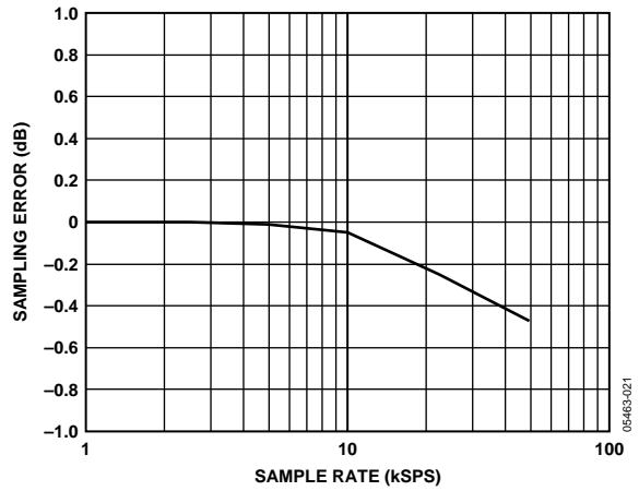
Figure 22. Sampling Error vs. Sample Rate
