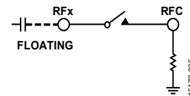
Figure 54. Series Capacitor Directly Connected to MEMS Switch
