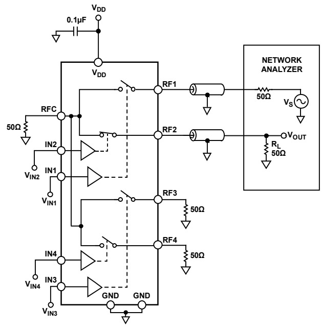
Figure 35. Crosstalk
