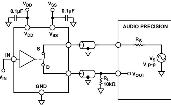
Figure 36. THD + N
