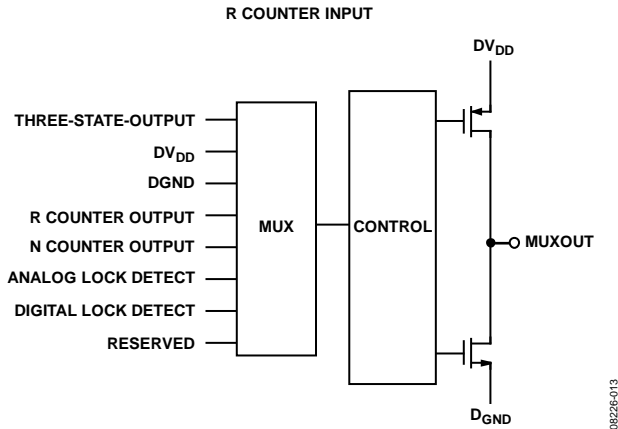
Figure 17. MUXOUT Schematic
