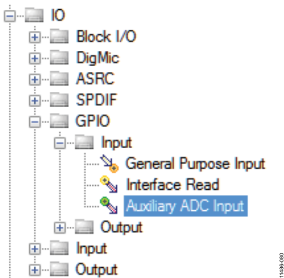
Figure 77. Auxiliary ADC Input Cell in the SigmaStudio Toolbox
