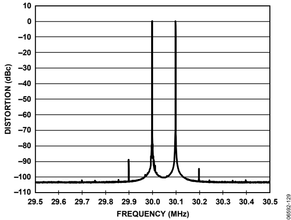
Figure 31. Intermodulation Distortion
