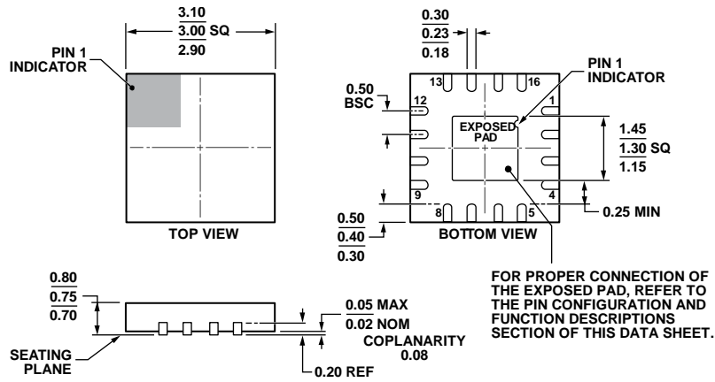
Figure 59. 16-Lead Lead Frame Chip Scale Package [LFCSP] 3 mm × 3 mm Body and 0.75 mm Package Height (CP-16-21)
