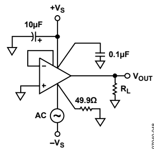
Figure 46. Negative Power Supply Rejection
