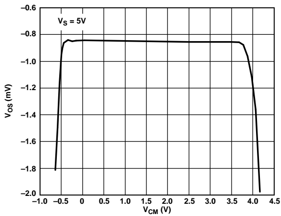
Figure 50. V OS vs. Common-Mode Voltage, V S = 5 V
