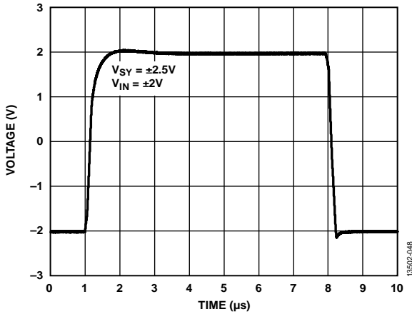
Figure 52. Large Signal Transient Response, V_{SV} = \pm 2.5V
