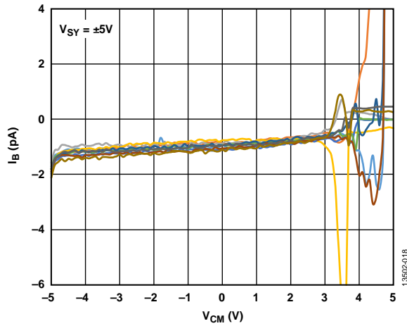
Figure 22. Input Bias Current ( I_B ) vs. Input Common-Mode Voltage ( V_{CM} ), V_{SY} = \pm 5 V
