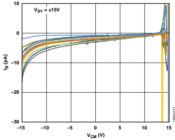
Figure 21. Input Bias Current ( I_B ) vs. Input Common-Mode Voltage ( V_{CM} ), V_{SY} = \pm 15 V
