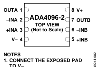
Figure 2. 8-Lead LFCSP (CP-8-10), ADA4096-2
