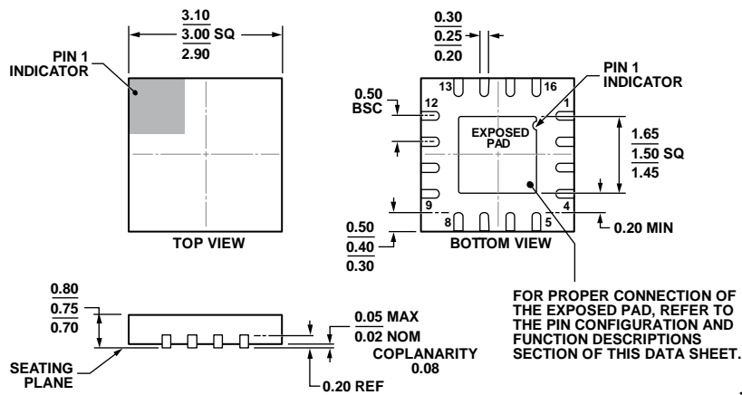
COMPLIANT TO JEDEC STANDARDS MO-220-WEED-6. Figure 60. 16-Lead Lead Frame Chip Scale Package [LF CSP_WQ] 3 mm x 3 mm Body, Very Very Thin Quad (CP-16-27) Dimensions shown in millimeters
