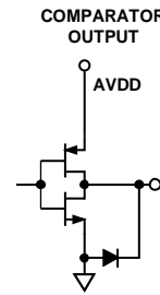
Figure 22. Comparator Outputs
