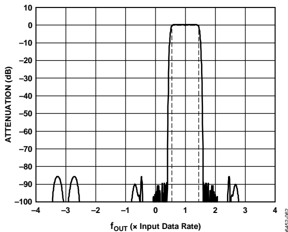
Figure 65. Interpolation/Modulation Combination of f_{DAC}/8 Filter
