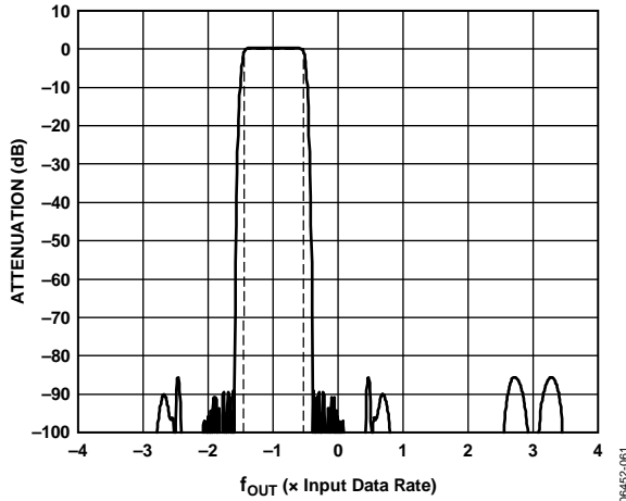
Figure 64. Interpolation/Modulation Combination of -f_{DAC}/8 Filter
