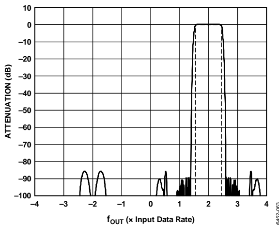
Figure 66. Interpolation/Modulation Combination of 2f_{DAC}/8 Filter
