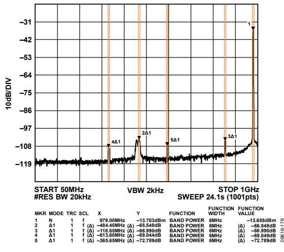
Figure 118. High Band Wideband ACLR
