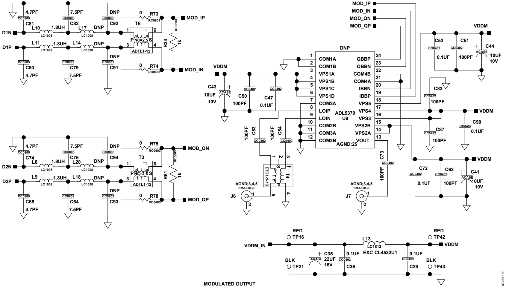
Figure 118. Modulated Output
