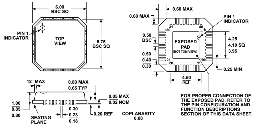
Figure 135. 40-Lead Lead Frame Chip Scale Package [LFCSP] 6 mm x 6 mm and 0.85 mm Package Height (CP-40-1)
