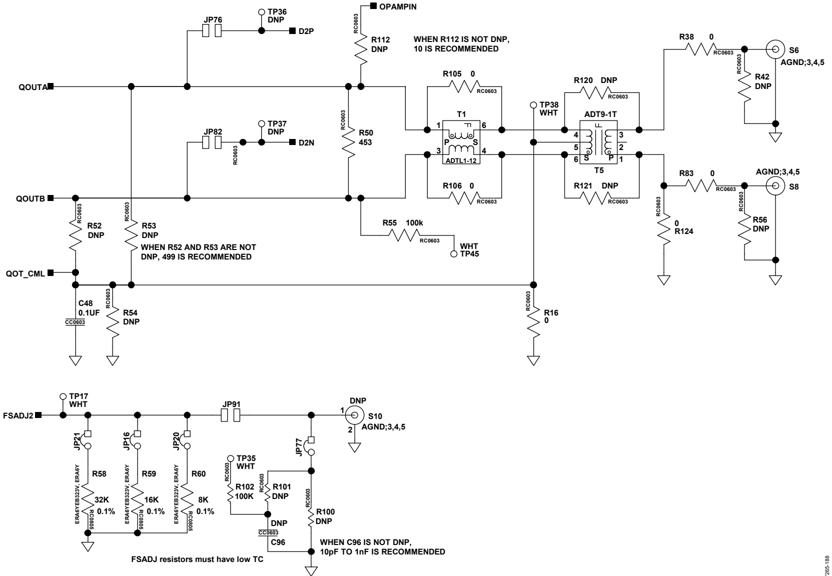
Figure 116. QOUT Network and FSADJ2
