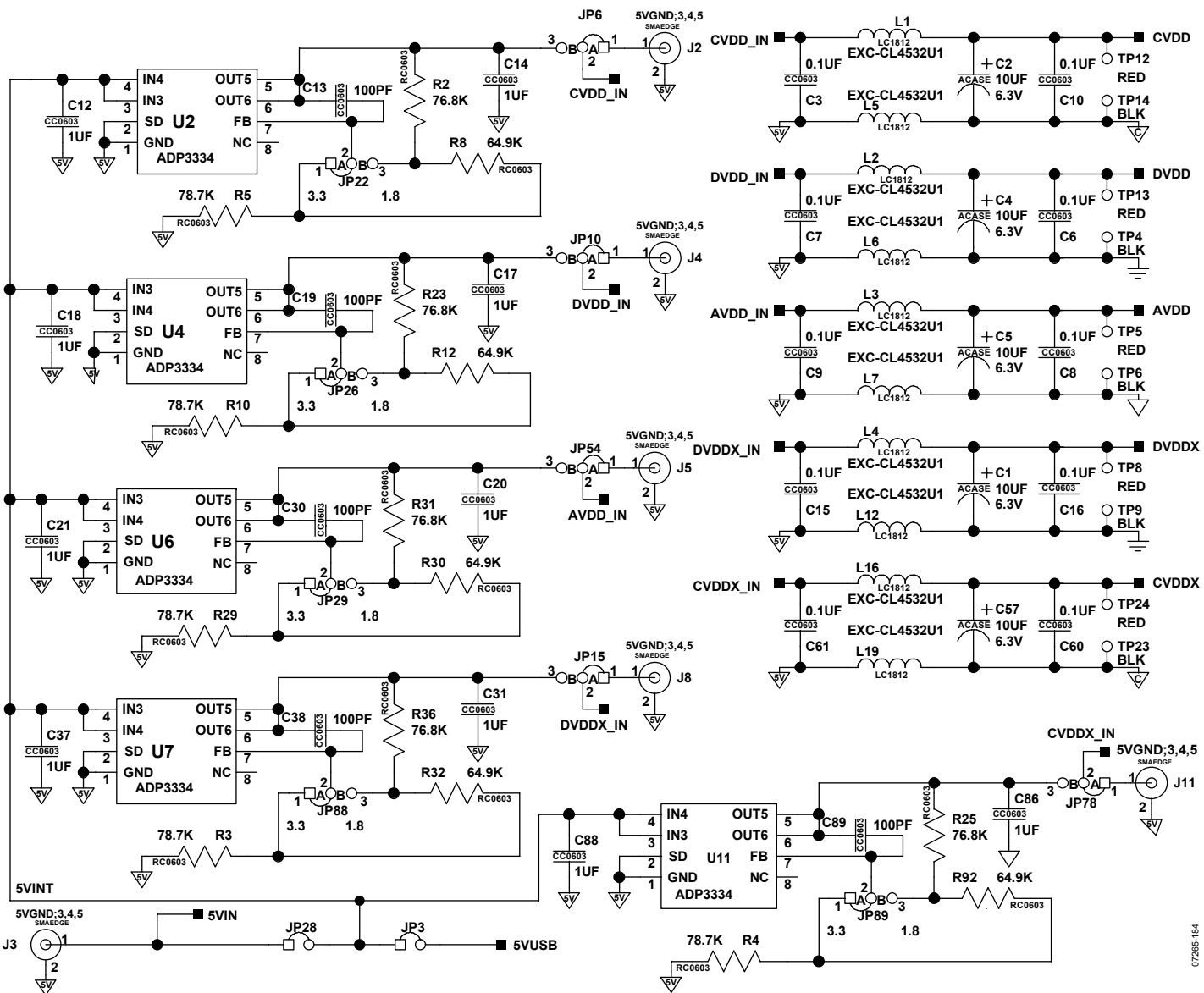
Figure 112. Power Supplies and Filters
