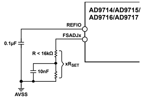
Figure 97. xRSET Configuration for Values > 16 kΩ
