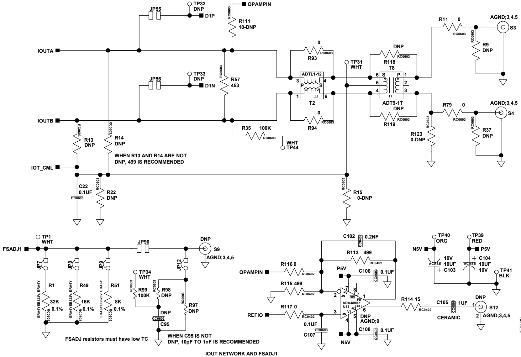
Figure 115. IOUT Network and FSADJ1
