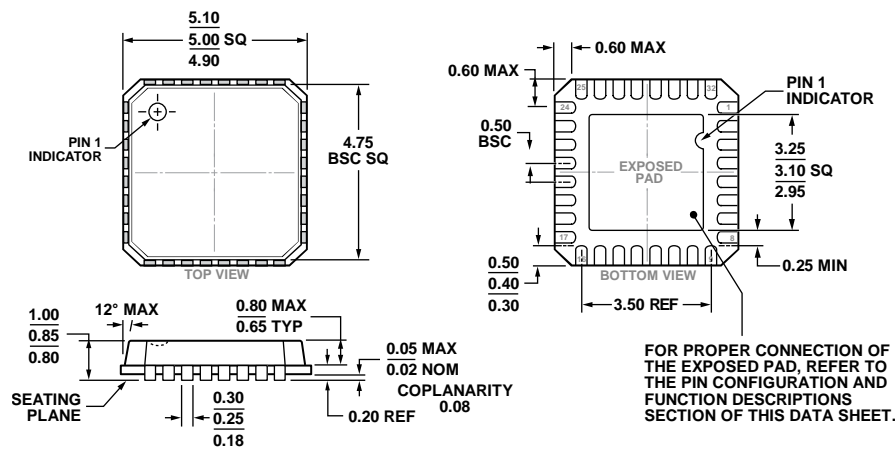
Figure 91. 32-Lead Lead Frame Chip Scale Package [LFCSF] 5 mm × 5 mm and 0.85 mm Package Height (CP-32-2) Dimensions shown in millimeters
