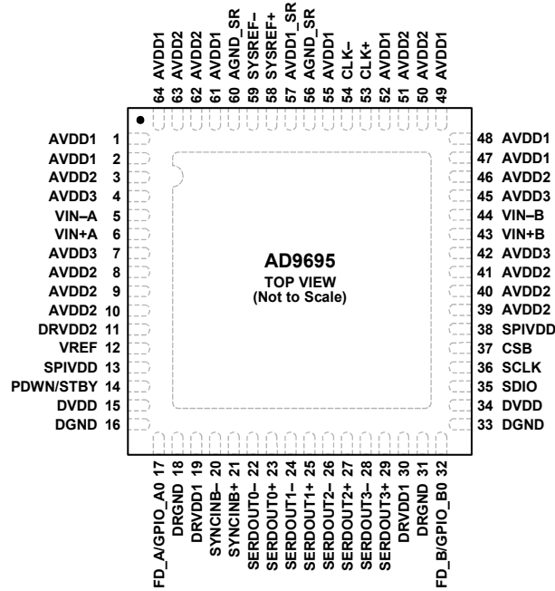
Figure 5. Pin Configuration (Top View)
