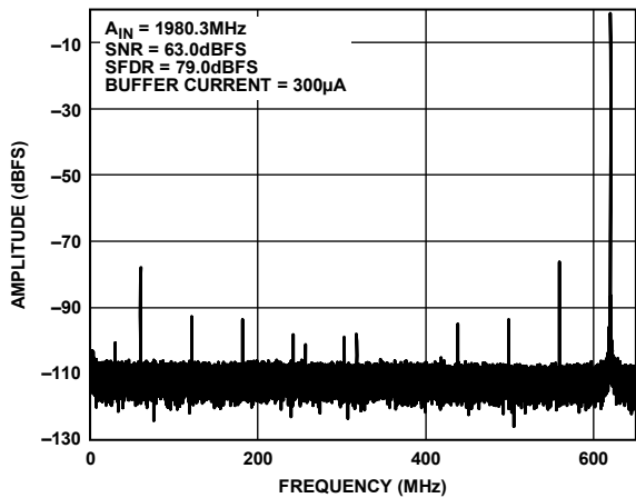
Figure 13. Single-Tone FFT with f_{IN} = 1980.3 MHz
