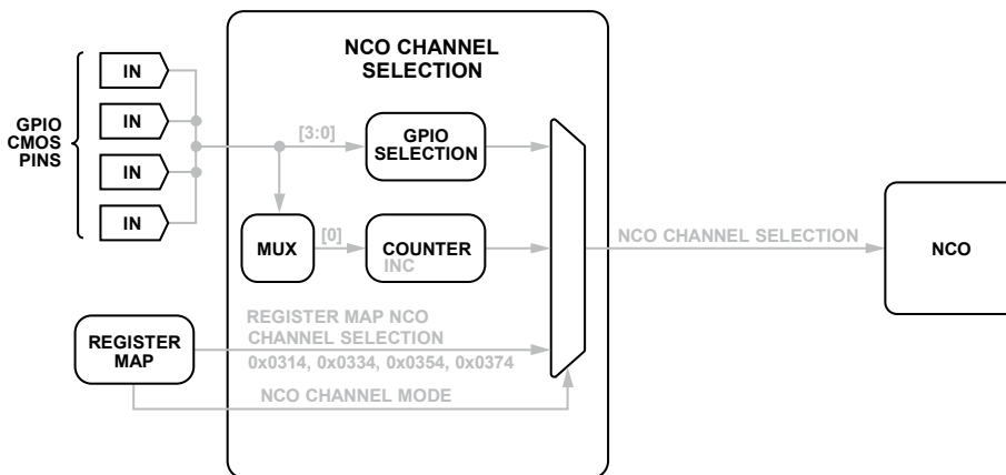
Figure 71. NCO Channel Selection Block
