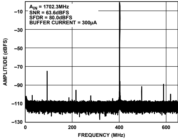
Figure 12. Single-Tone FFT with f_{IN} = 1702.3 MHz
