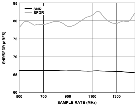
Figure 14. SNR/SFDR vs. Sample Rate, f_{IN} = 172.3 MHz
