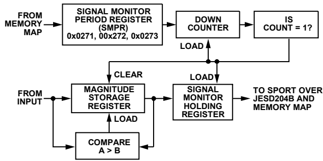
Figure 82. Signal Monitor Block
