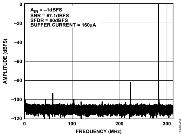
Figure 34. Single-Tone FFT with f_{IN} = 340 MHz
