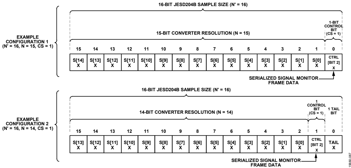
Figure 83. Signal Monitor Control Bit Locations
