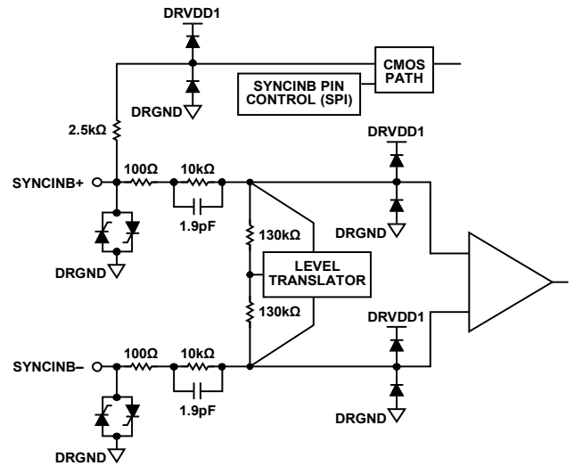
Figure 61. SYNCINB± Inputs
