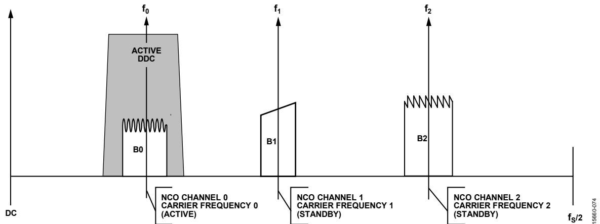
Figure 72. NCO Coherent Mode with Three NCO Channels (B0 Selected)
