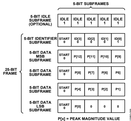
Figure 84. SPORT over JESD204B Signal Monitor Frame Data
