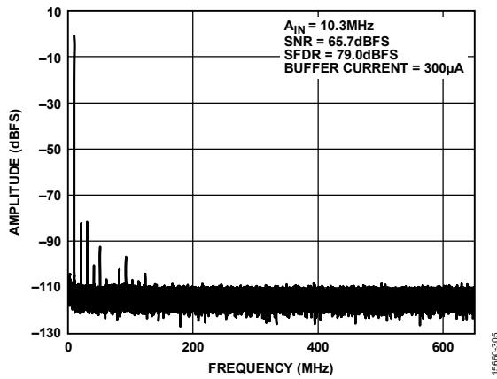
Figure 6. Single-Tone FFT with Analog Input Frequency ( f_{IN} ) = 10.3 MHz
