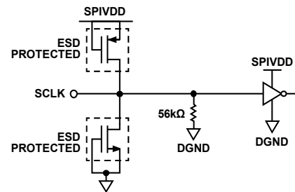
Figure 62. SCLK Input
