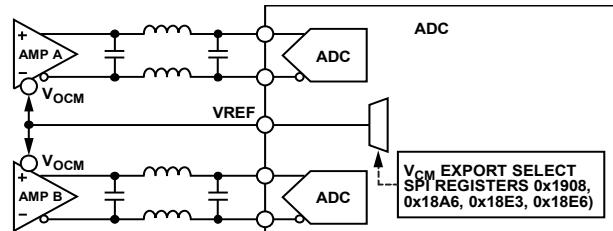
Figure 70. DC-Coupled Application Using the AD9695
