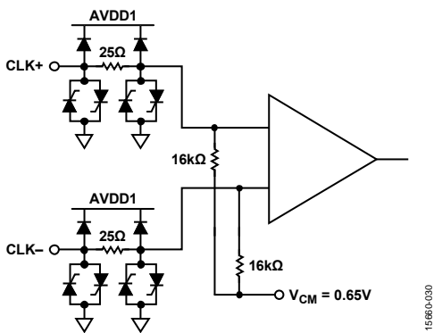
Figure 58. Clock Inputs
