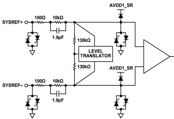
Figure 59. SYSREF± Inputs
