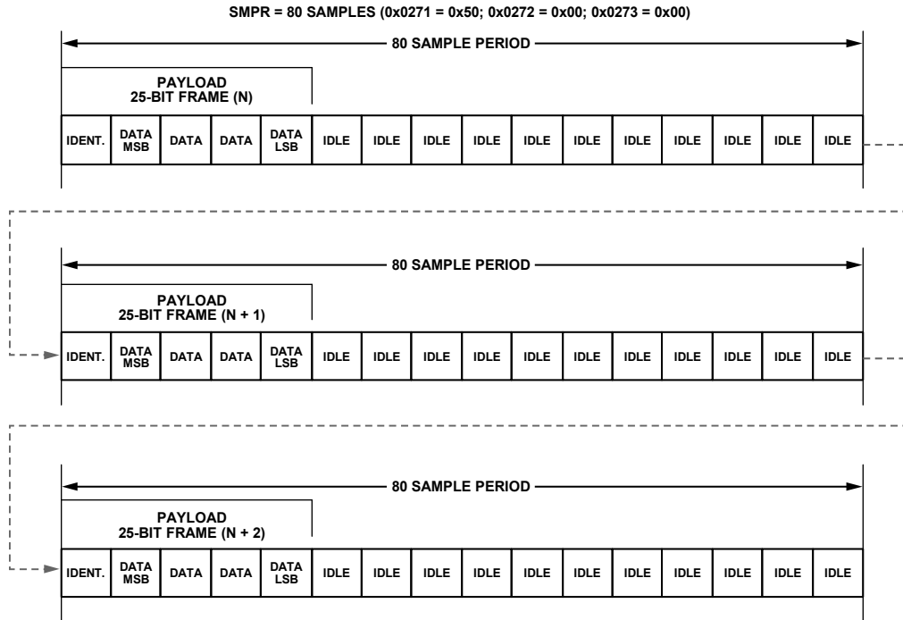
Figure 85. SPORT over JESD204B Signal Monitor Example
