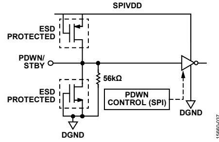
Figure 65. PDWN/STBY Input
