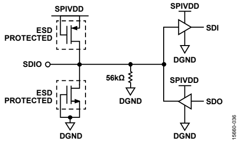
Figure 64. SDIO Input
