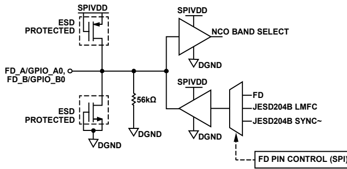
Figure 67. FD_A/GPIO_A0 and FD_B/GPIO_B0
