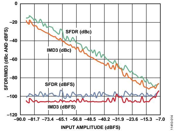
Figure 14. AD9683-170 Two-Tone SFDR/IMD3 vs. Input Amplitude ( A_{IN} ) with f_{IN1} = 184.12\text{ MHz} , f_{IN2} = 187.12\text{ MHz} , f_S = 170\text{ MSPS}
