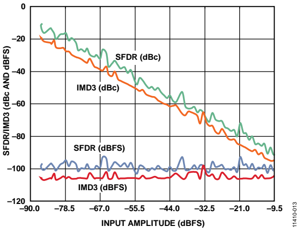
Figure 13. AD9683-170 Two-Tone SFDR/IMD3 vs. Input Amplitude ( A_{IN} ) with f_{IN1} = 89.12\text{ MHz} , f_{IN2} = 92.12\text{ MHz} , f_S = 170\text{ MSPS}
