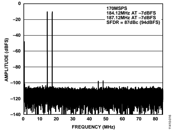
Figure 16. AD9683-170 Two-Tone FFT with f_{IN1} = 184.12\text{ MHz} , f_{IN2} = 187.12\text{ MHz} , f_S = 170\text{ MSPS}
