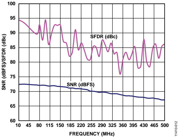
Figure 12. AD9683-170 Single-Tone SNR/SFDR vs. Input Frequency ( f_{IN} ), RFCLK = 680\text{ MHz} with Divide by 4 (Address 0x09 = 0x21 )
