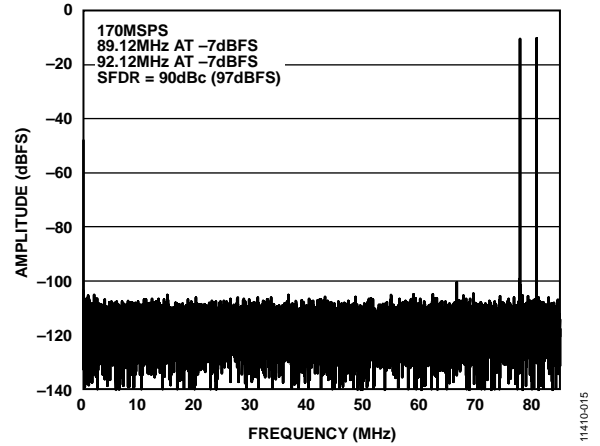
Figure 15. AD9683-170 Two-Tone FFT with f_{IN1} = 89.12\text{ MHz} , f_{IN2} = 92.12\text{ MHz} , f_S = 170\text{ MSPS}
