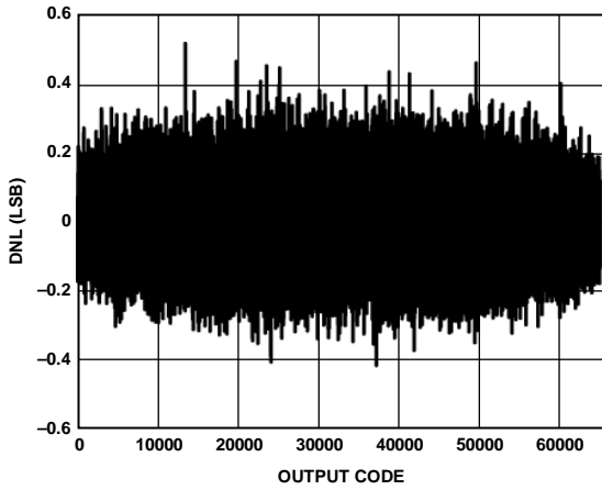
Figure 17. Differential Nonlinearity (DNL), f_{IN} = 9.7 MHz, f_{SAMPLE} = 125 MSPS, V_{REF} = 1.4 V
