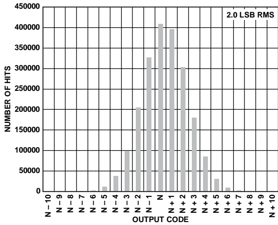
Figure 18. Input Referred Noise Histogram, f_{SAMPLE} = 125 MSPS, V_{REF} = 1.4 V
