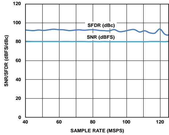
Figure 19. SNR/SFDR vs. Sample Rate, f_{IN} = 9.7 MHz, V_{REF} = 1.4 V
