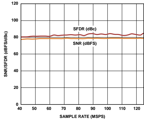
Figure 20. SNR/SFDR vs. Sample Rate, f_{IN} = 64 MHz, V_{REF} = 1.4 V
