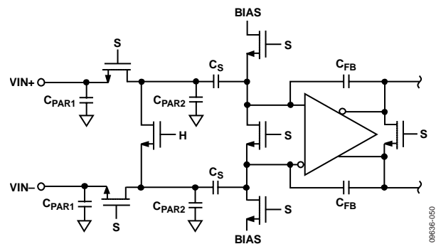
Figure 46. Switched-Capacitor Input
