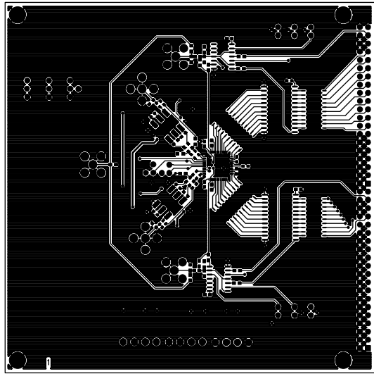
Figure 29. Top Routing
