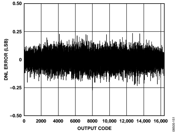
Figure 51. AD9255-125 DNL with f_{IN} = 12.5 MHz
