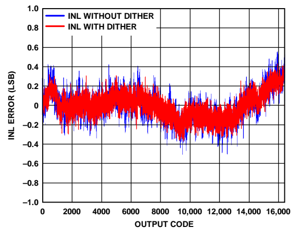
Figure 28. AD9255-105 INL with f_{IN} = 12.5 MHz
