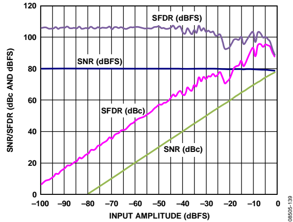
Figure 39. AD9255-125 Single-Tone SNR/SFDR vs. Input Amplitude ( A_{IN} ) with f_{IN} = 2.4 MHz
