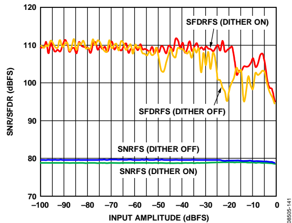
Figure 41. AD9255-125 Single-Tone SNR/SFDR vs. Input Amplitude ( A_{IN} ) with f_{IN} = 30 MHz With and Without Dither Enabled
