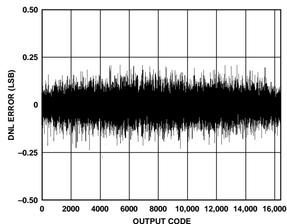
Figure 29. AD9255-105 DNL with f_{IN} = 12.5 MHz
