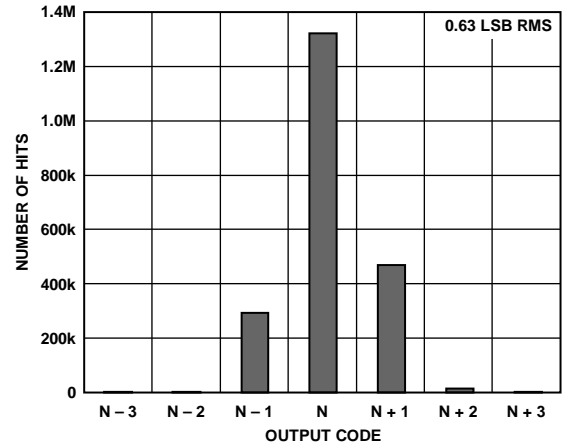
Figure 27. AD9255-105 Grounded Input Histogram
